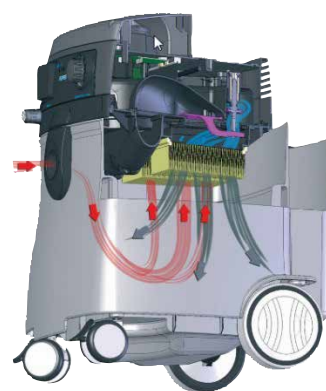
Air cycle during filter cleaning
