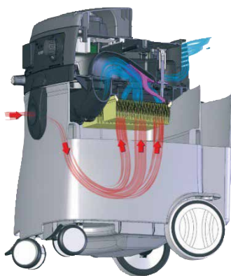
Air cycle during normal operation
